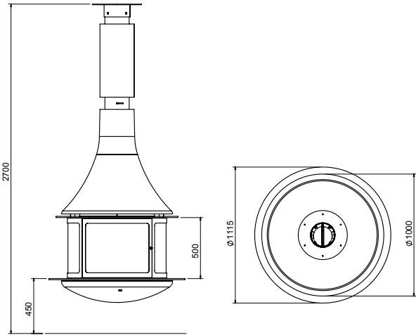
LORENA CENTRAL SUSPENDIDA CON CERRAMIENTO. LORENA SUSPENDED CENTRAL WITH CLOSING SYSTEM. LORENA CENTRAL SUSPENDUE FOYER FERMÉ.
