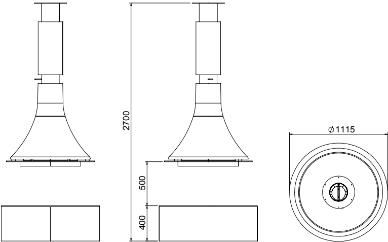
LORENA CENTRAL SUSPENDIDA SIN CERRAMIENTO. LORENA SUSPENDED CENTRAL WITHOUT CLOSING SYSTEM. LORENA CENTRAL SUSPENDUE FOYER OUVERT.
